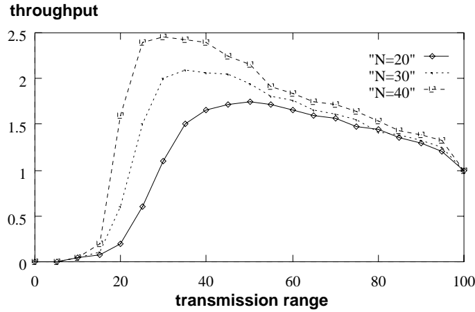
Figure 19: End-to-end throughput
